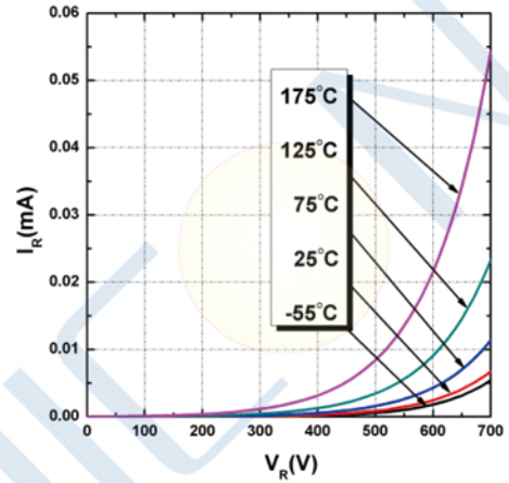
Figure 2. Reverse Characteristics
