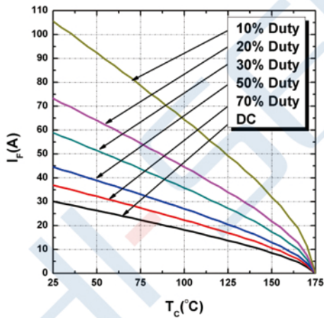
Figure 3. Current Derating
