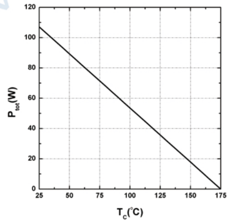
Figure 4. Power Derating
