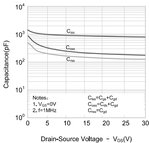
Figure 5. Capacitance Characteristics
