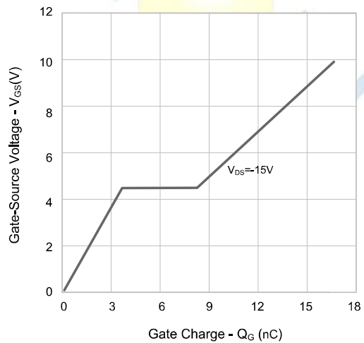
Figure 6. Gate Charge
