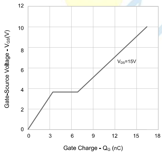
Figure 6. Gate Charge
